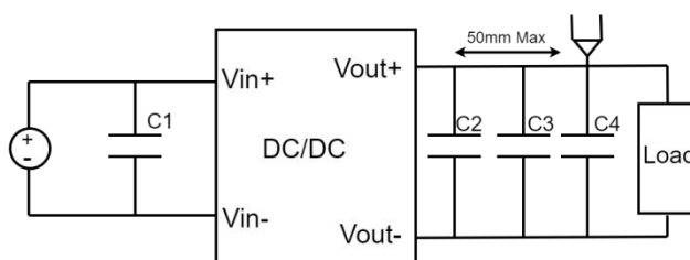
Fig.2 Schematic diagram of output ripple voltage
