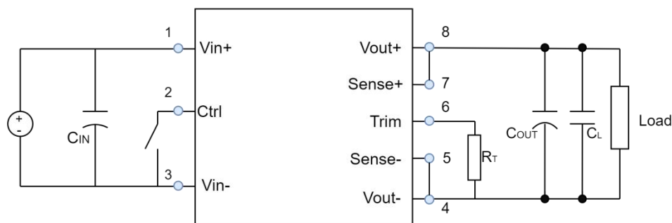
Fig. 6 Output Voltage Forward Regulation
