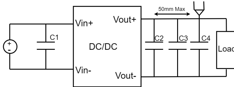
Fig.2: Schematic diagram of output ripple voltage
