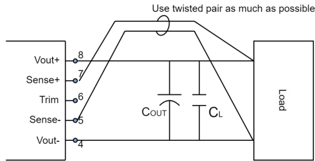
Fig. 5 Schematic Diagram of Sense Terminal Wiring
