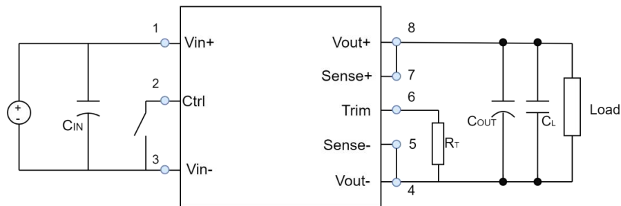
Fig. 6 Output Voltage Forward Regulation
