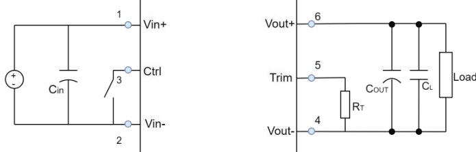
Fig 4: Functional application diagram of Trim
