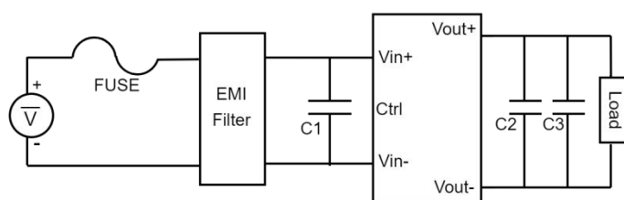
Fig. 1 Single-channel Typical Application Diagram
