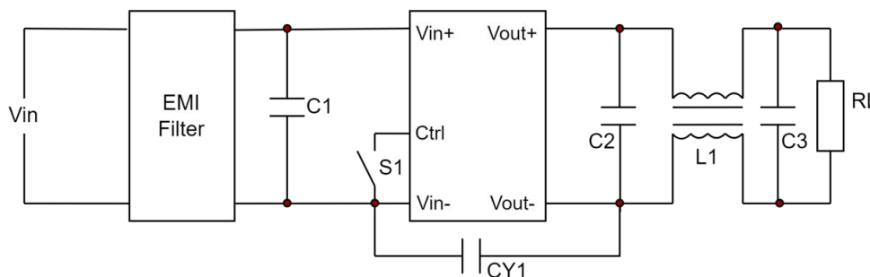
Fig.2 Link diagram of EMI filter circuit
