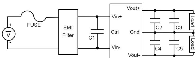
Fig. 2 Dual-channel Typical Application Diagram
