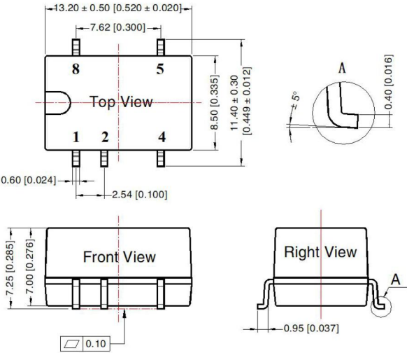
Figure 7: Overall dimensions
