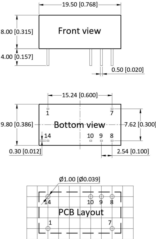
Figure 7: Overall dimensions
