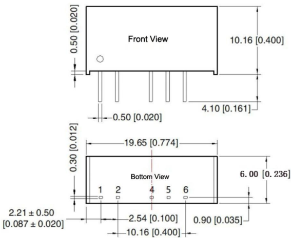
Figure 7: Overall dimensions
