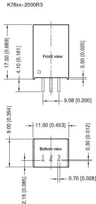
Figure 7: Overall dimensions
