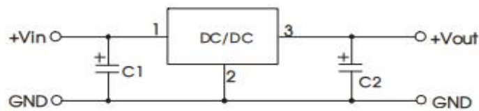
Figure 1: Application circuit
