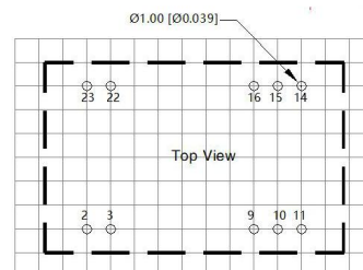
PCB Printing Layout
