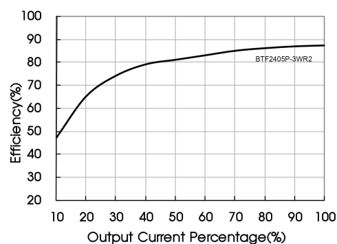
Efficiency VS Output Load (Vin=24V)
