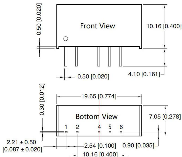
Figure 7: Overall dimensions
