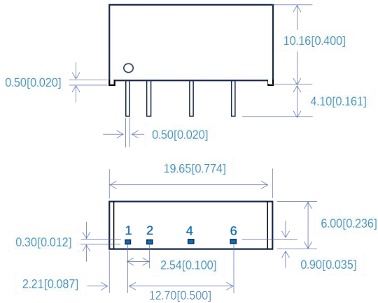
Figure 7: Overall dimensions
