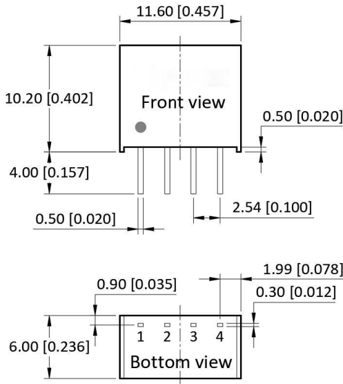
Figure 7: Overall dimensions
