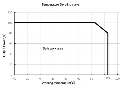
Figure 4: Temperature Derating Curve
