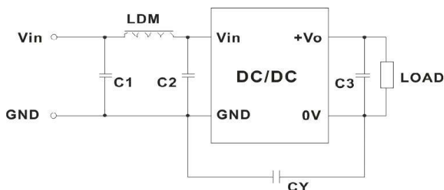
Figure 2: EMC Typical Recommended Circuits
