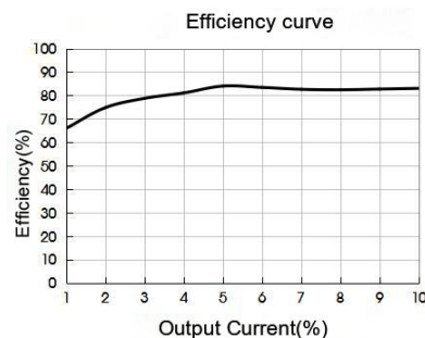
Figure 5: Efficiency VS Output Load (Nominal Voltage Input)
