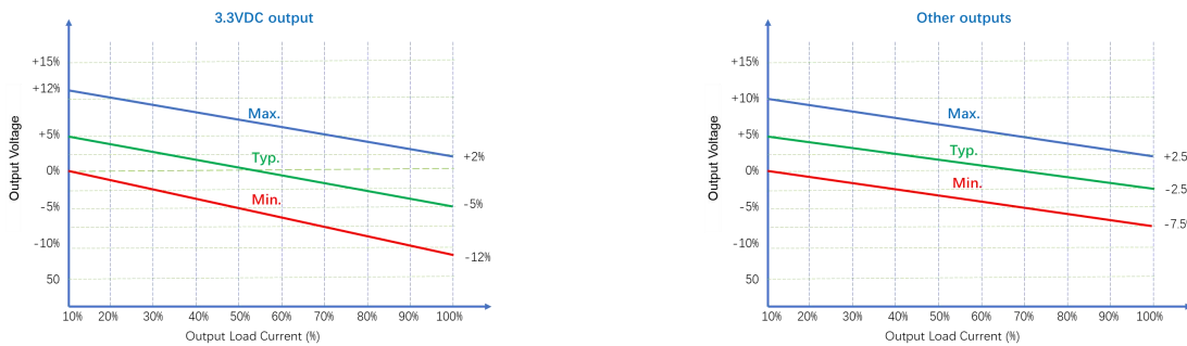
Figure 3: Voltage tolerance envelope
