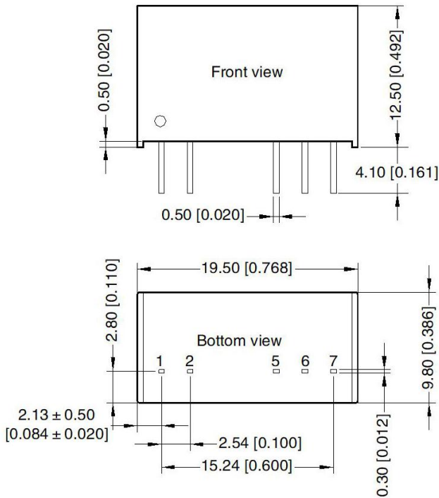
Figure 7: Overall dimensions
