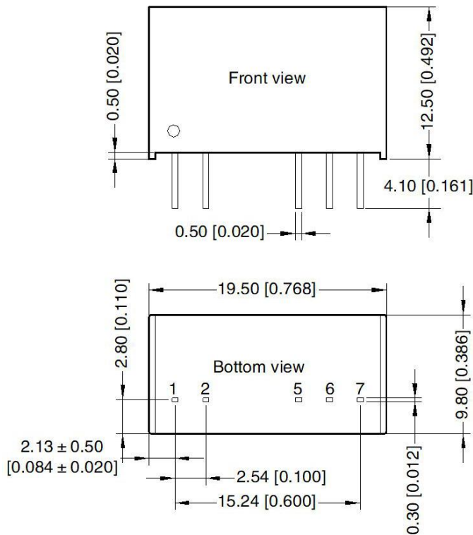
Figure 7: Overall dimensions
