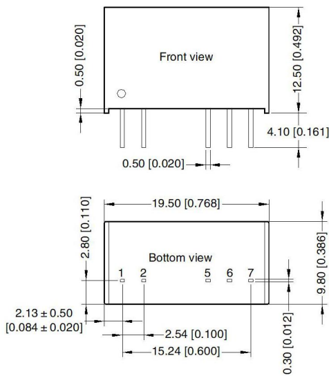
Figure 7: Overall dimensions
