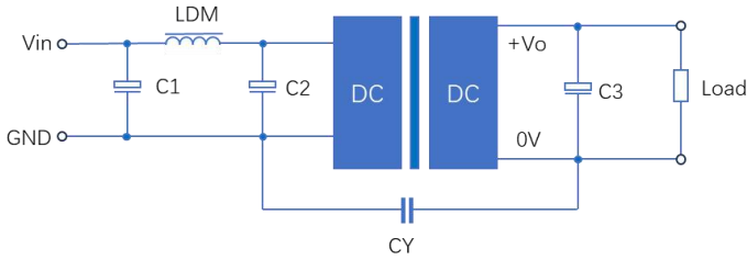
Figure 2: EMC Typical Recommended Circuits
