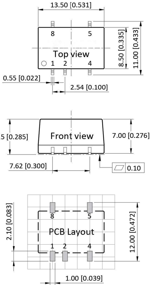
Figure 7: Overall dimensions
