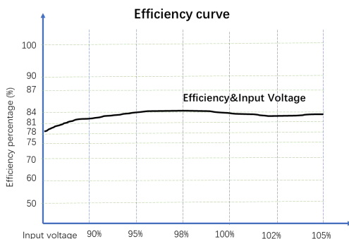
Figure 6: Efficiency VS Input Voltage (100% Load)
