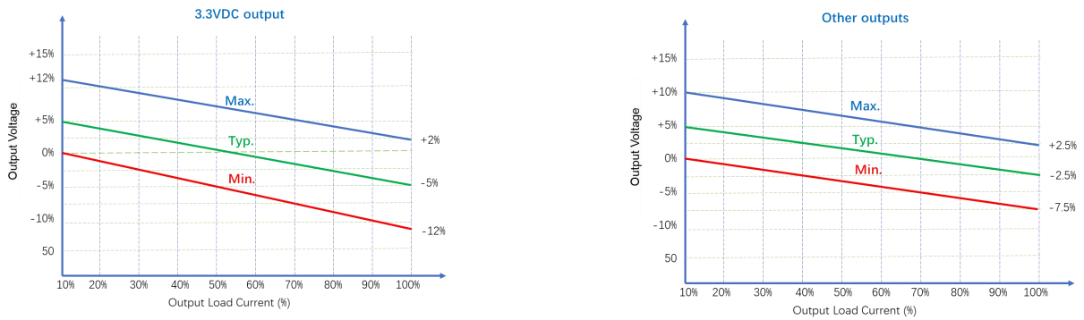
Figure 3: Voltage tolerance envelope
