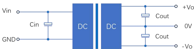
Figure 1: Application circuit
