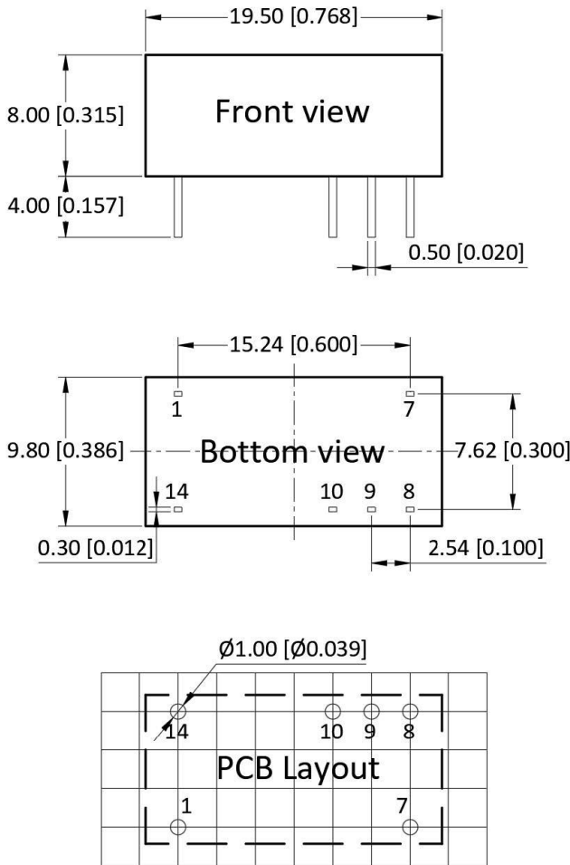
Figure 7: Overall dimensions
