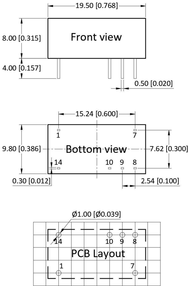
Figure 7: Overall dimensions
