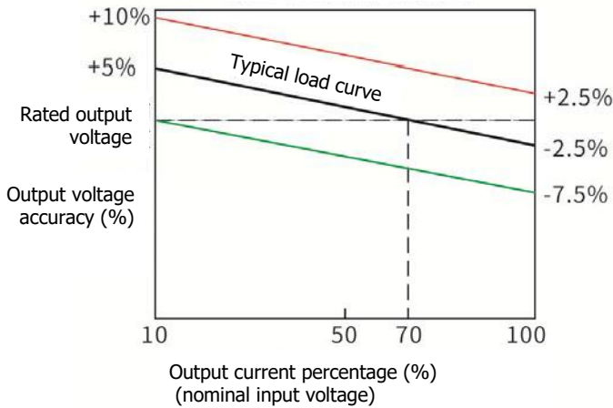
Load curve
