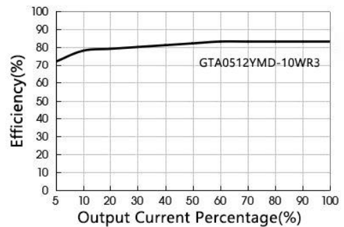
Efficiency Vs Output Load(Vin=5V)
