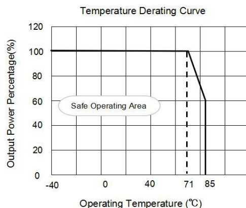
Temperature Derating Curve (Figure 1)
