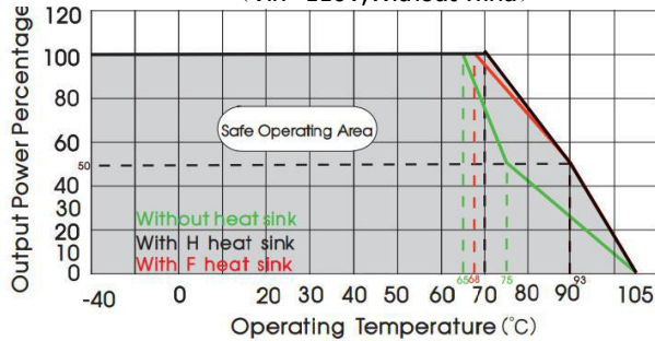
ATH1D03/05/12LD-20W(H/F)R3 temperature derating curve (Vin=110V, Without wind)
