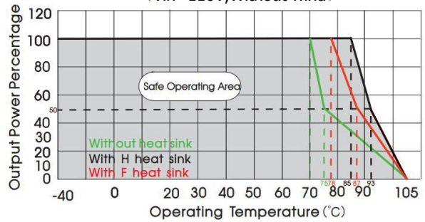
ATH1D24/48/54LD-20W(H/F)R3 temperature derating curve (Vin=110V, Without wind)
