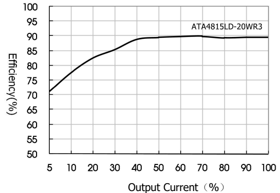
Efficiency Vs Output Load (Vin=24V)
