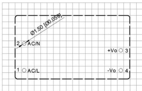
Recommended Footprint
