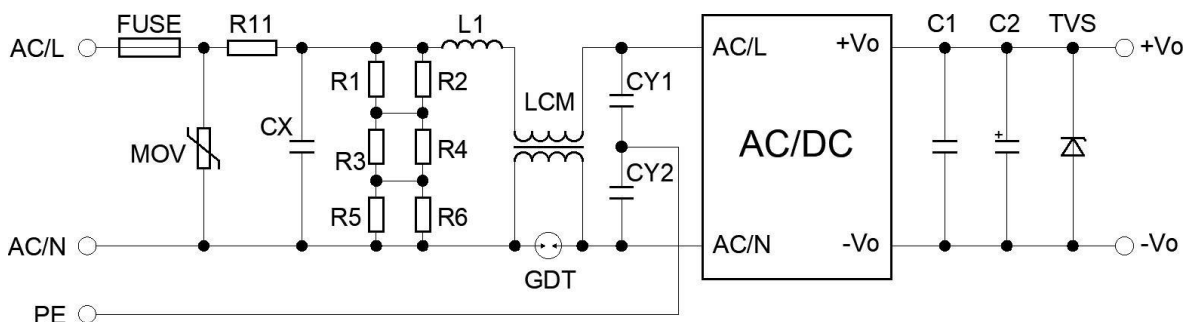
Figure 1. Circuit for EMC Enhancement
