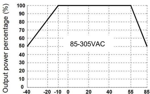
Temperature Derating Curve
