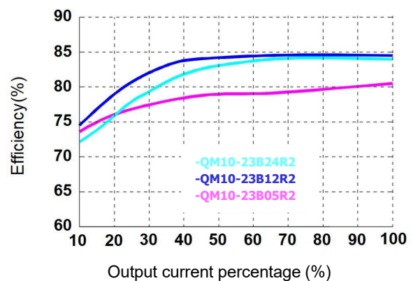
Efficiency VS out load (Vin=230VAC)
