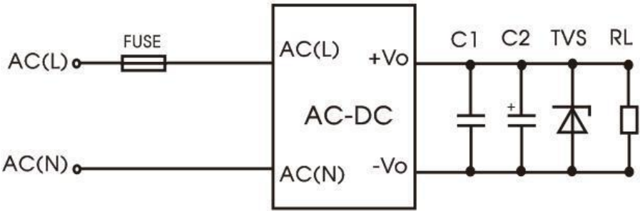
Recommended Peripheral Components
