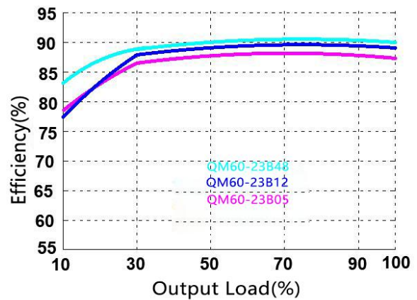
Efficiency Vs Output Load Derating Curve
