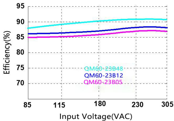
Efficiency Vs Input Voltage Derating Curve
